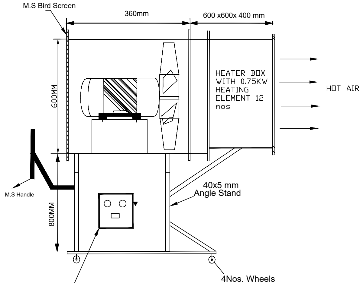
FRONT - VIEW
